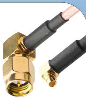
RA SMA Plug Right Angle Plug to RA MMCX Plug Right Angle Plug RG316 Cable
