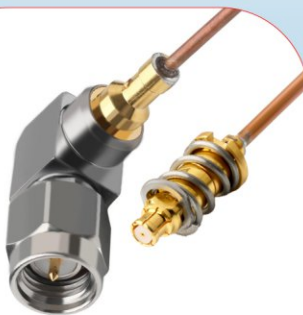
VITA 67 SMPM Straight Cable Jack SMA Male Straight Angle Plug SR047 SEMI-RIGID Cable
