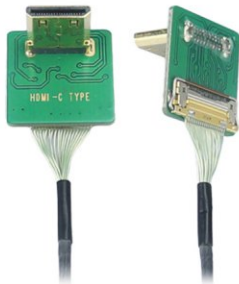
MINI-HDMI elbow head HDMI-C2 to IPEX 20525-020E-02
