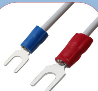
SVM2-4 TO SVM1.25-4 TERMINAL CABLE
