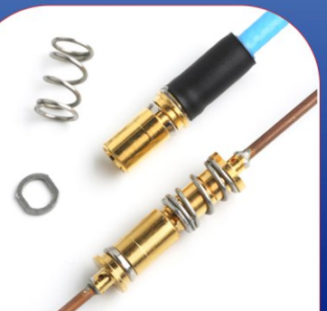
RG SMA Male to SMA Jack 0.085 Flexible Coax
